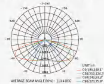
Meridian Light Distribution Curve(40W Parameter)
